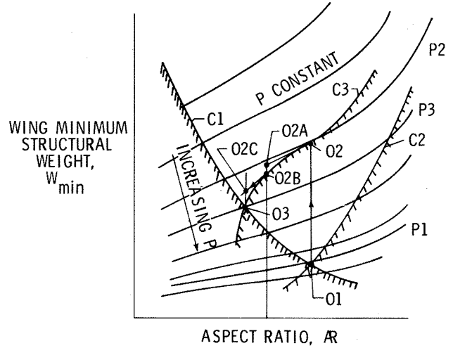
FIGURE 6 A PATH TOWARD NEW CONSTRAINED MINIMUM
