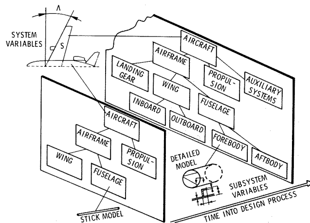
FIGURE 13 DECOMPOSITION ADAPTS TO DESIGN STAGE
