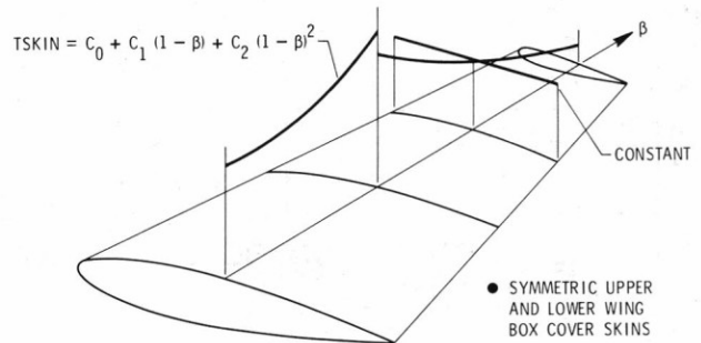
FIGURE 18 SKIN THICKNESS DISTRIBUTION, SIMPLIFIED FOR INITIAL TESTING
