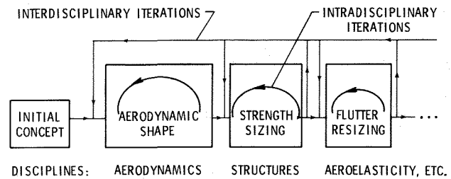
FIGURE 1 SEQUENTIAL DECISIONS IN DESIGN
