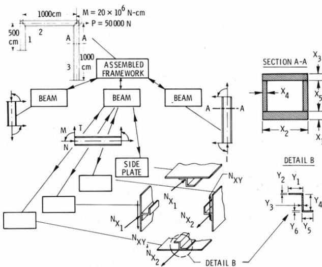
FIGURE 15 THREE-LEVEL FRAMEWORK TEST
