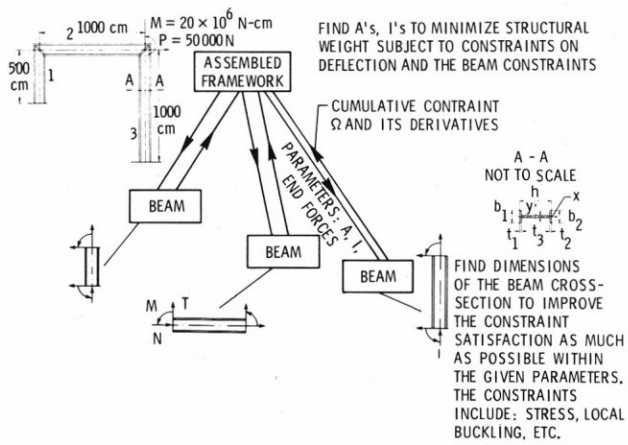
FIGURE 14 TWO-LEVEL FRAMEWORK TEST
