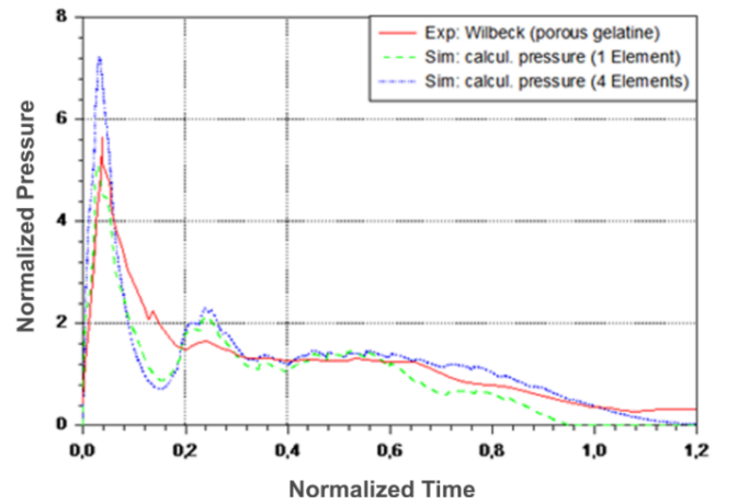
Fig. 1. Pressure in a porous gelatin projectile high velocity impact [8].
