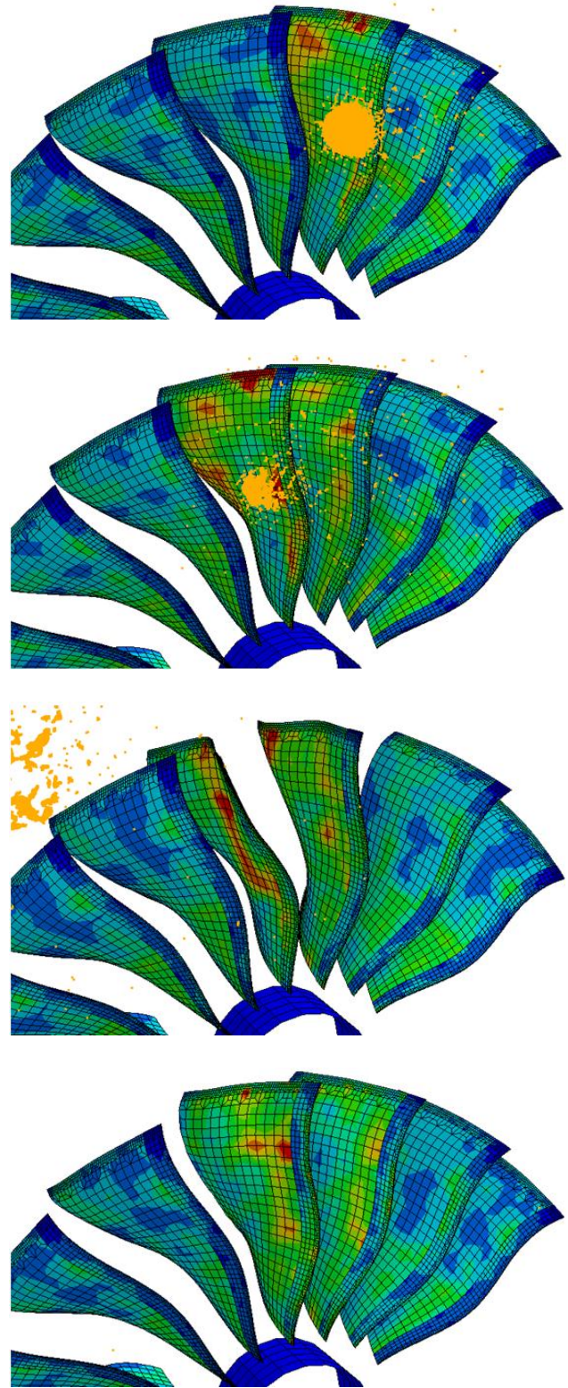
Fig. 18. von Mises stresses induced by the bird impact at progressive time steps.
