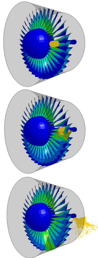
Fig. 8. Impact between the bird and fan assembly.
