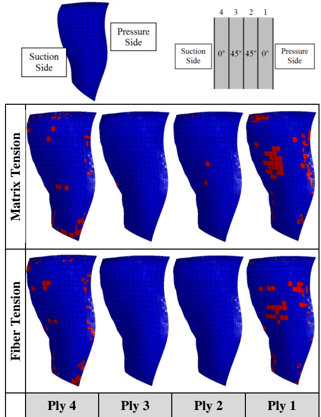
Fig. 21. Matrix and fiber tensile damage within each layer for an impacted hybrid fan blade.
