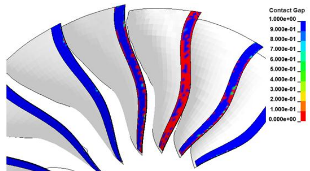
Fig. 22. Leading edge delamination following bird impact.
