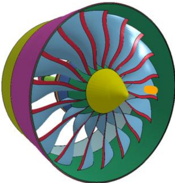
Fig. 23. Forward section bird impact scenario with hybrid fan blades
