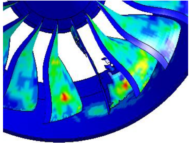
Fig. 24. Hybrid blade failure from 8 lb. bird impact.
