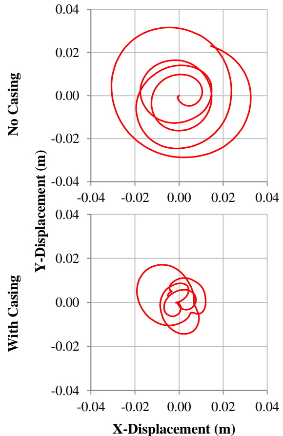
Fig. 11. Center hub displacement orbit plots.
