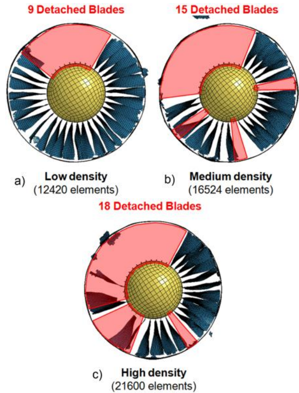
Fig. 14. Damage after several rotations for (a) 12420, (b) 16524, and (c) 21600 blade elements.
