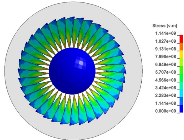
Fig. 5. Fan assembly stresses following the pre-stressing phase.
