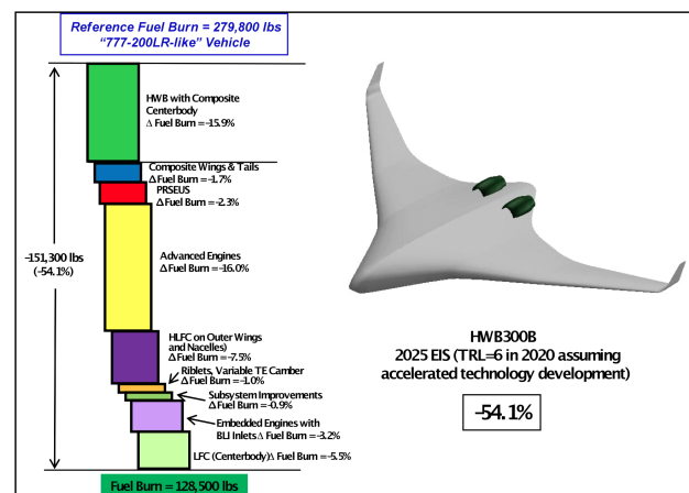
Fig. 5 – Advanced Hybrid Wing Body HWB300B waterfall chart.
