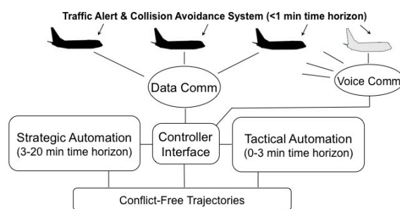
Figure 1. Trajectory automation system top level diagram
