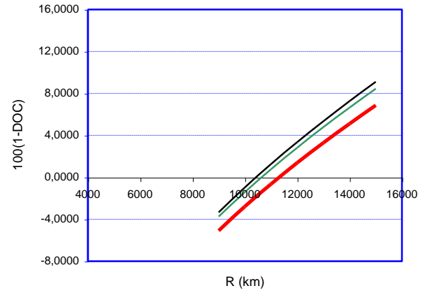
Figure 10. Relative DOC variations when the route is split into two segments of 60 and 50 percent the original distance, for PL=30000 kg. — current cost sharing; — 50% increased fuel prices; — increased fuel prices plus eco-tax.
