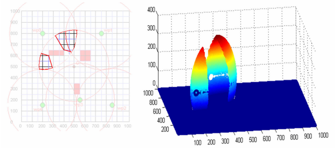
Fig 13. The first CFOV has been calculated. Left: a sketch of the areas. Right: A 3D visualization of the same areas. The plot is hollow since only zmin and zmax is shown..
