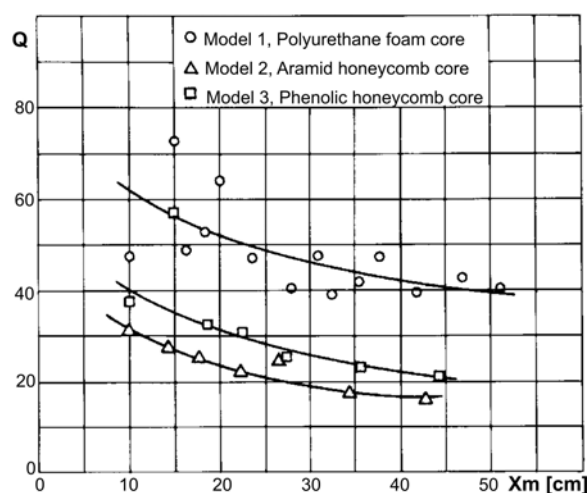
Fig. 14: Q -factor of blade vibration for all three types of models
