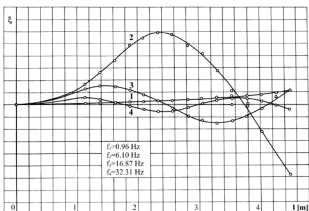
Fig. 6: Natural modes of oscillation for the blade with Rohacell polyurethane foam core (Model 1)
