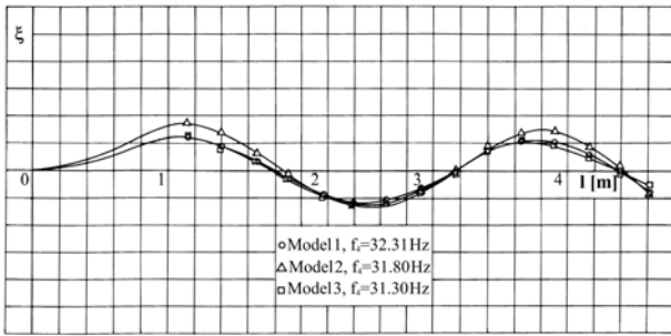
Fig. 9: Comparative results for the third oscillation mode
