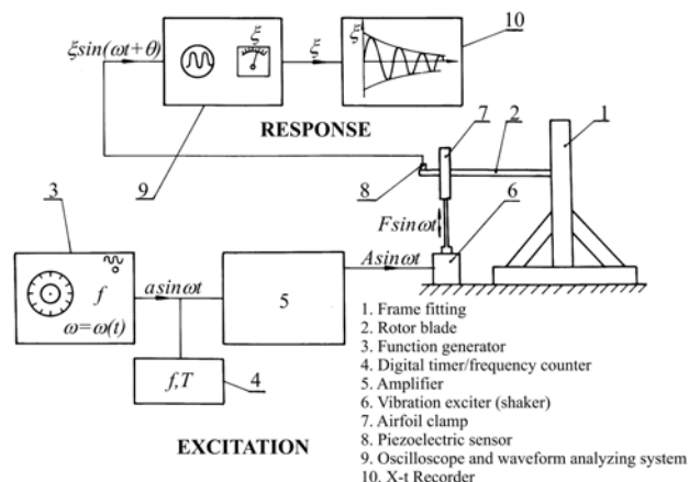
Fig. 5: Employed equipment in vibratory testing
