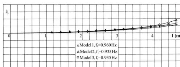
Fig. 7: Comparative results for the first oscillation mode
