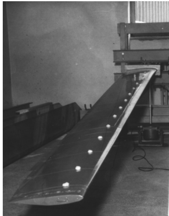
Fig. 4: The main rotor blade in vibratory testing
