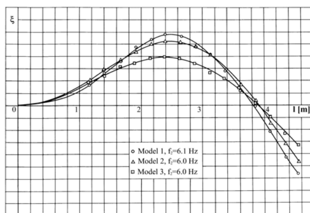
Fig. 8: Comparative results for the second oscillation mode
