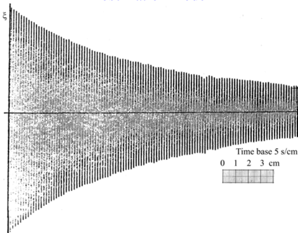
Fig. 10: Comparative results for the fourth oscillation mode
