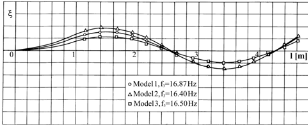
Fig. 9: Comparative results for the third oscillation mode
