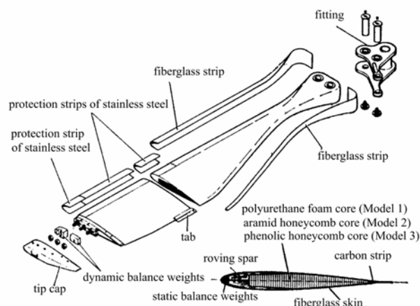
Fig. 2: The helicopter main rotor blade made of composite laminated materials
