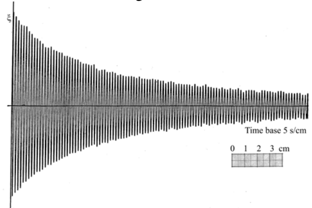
Fig. 12: Structural damping for the blade with Nomex phenolic honeycomb core (Model 3)
