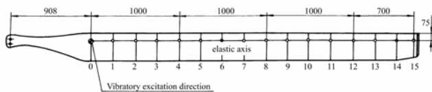
Fig. 3: Measurement points in vibratory testing
