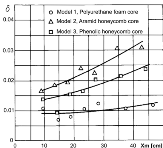
Fig. 13: Logarithmic decrement of blade free vibration
