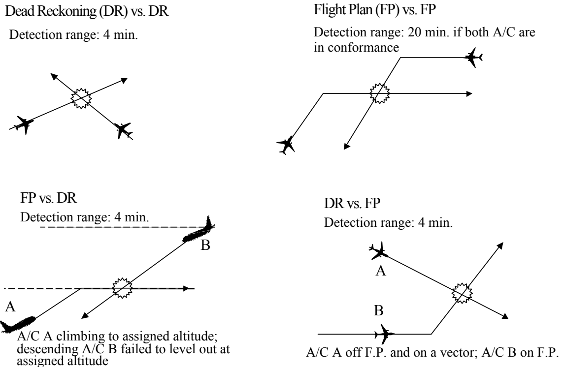
Fig. 3 Multi-trajectory conflict detection
