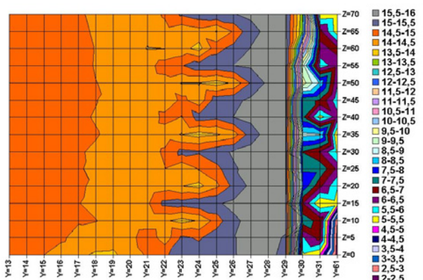
Fig.10. Topography of airfoil with ST3% at Re_y = 350000 . \alpha = 10 -deg and flap at 12-deg.
