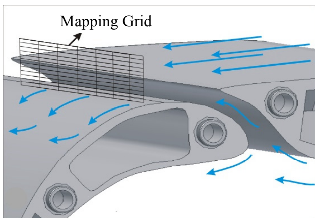
Fig.03. Mapping grid of the hot wire anemometry measurements.
