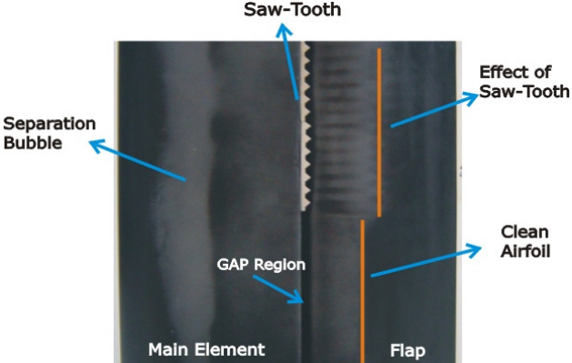
Fig.15. Visualization effect of saw-tooth and clean airfoil over upper surface flap at Re = 400000 . \alpha = 10 -deg and flap at 12-deg.
