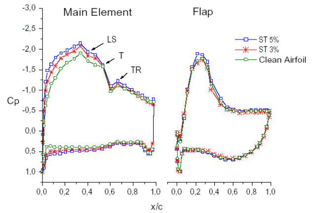
Fig. 07. C_p vs. x/c at 4-deg incidence angle and flap at 4-deg. Comparison of different saw-tooth configurations and clean airfoil for Re_y = 395000 .
