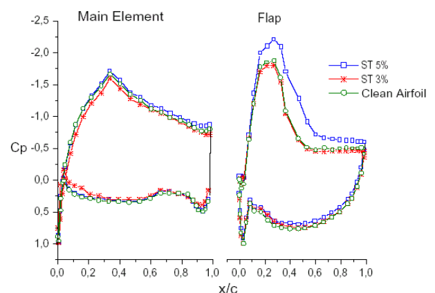
Fig. 05. C_p vs. x/c at -2-deg incidence angle and 8-deg flap angle. Comparison of different saw-tooth configurations and clean airfoil for Re_y = 390000 .
