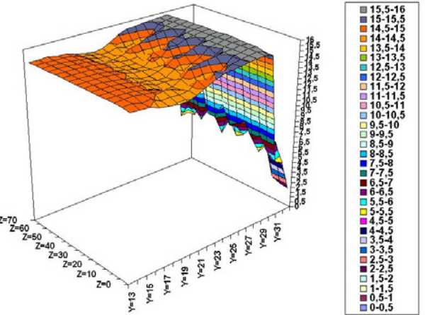
Fig.12. Three-dimensional of airfoil with ST3% at Re = 350000 . \alpha = 10 -deg and flap at 12-deg.
