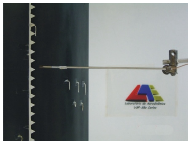
Fig.04. Hot wire anemometer measurements.
