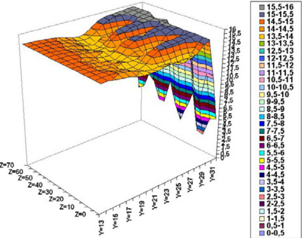
Fig.13. Three-dimensional of airfoil with ST5% at Re = 350000 . \alpha = 10 -deg and flap at 12-deg.
