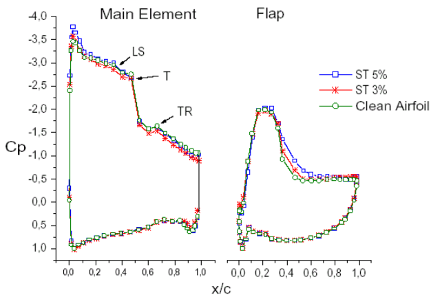
Fig. 06. C_p vs. x/c at 10-deg incidence angle and flap at 8-deg. Comparison of different saw-tooth configurations and clean airfoil for Re_y = 380000 .
