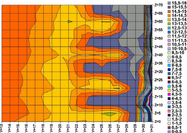
Fig.11. Topography of airfoil with ST5% at Re = 350000 . \alpha = 10 -deg and 12-deg flap angle.
