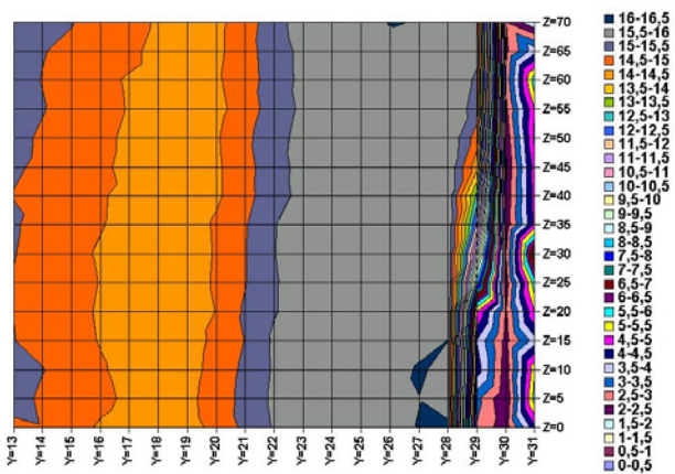
Fig. 09. Topography of clean airfoil at Re_y = 350000 . \alpha = 10 -deg and flap at 12-deg.
