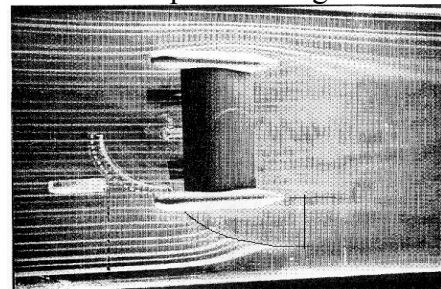
Figure 5 Flow visualization with smoke stream
