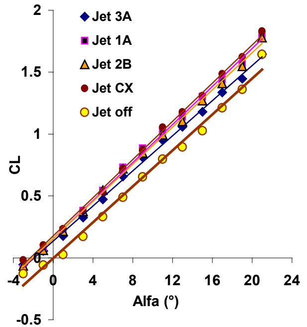
Figure 10 Double Jets Lift to alpha curves.
