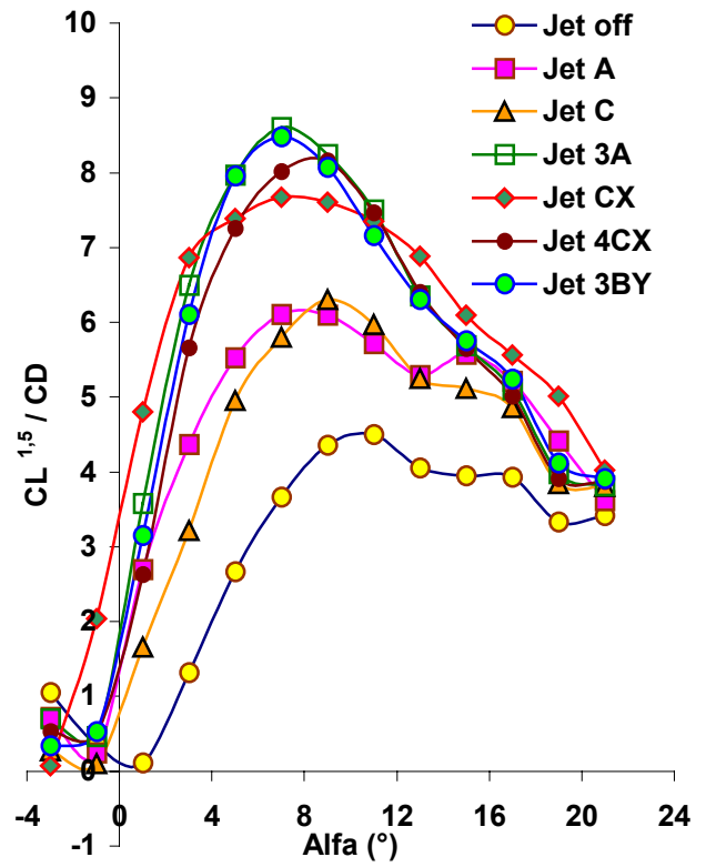
Figure 17 Climb rate factor results of the best configurations.
