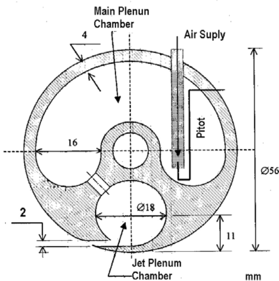
Figure 3 Jet module geometry and dimensions
