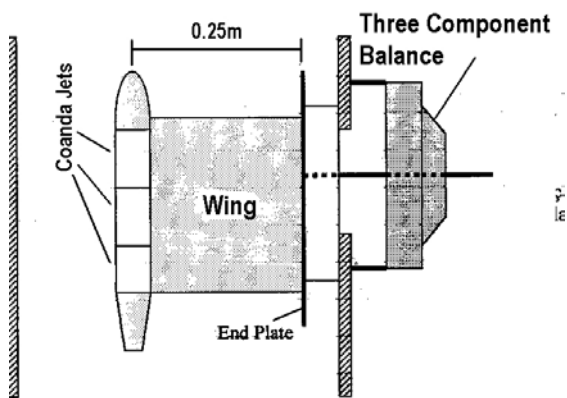
Figure 2 Experimental Set-up
