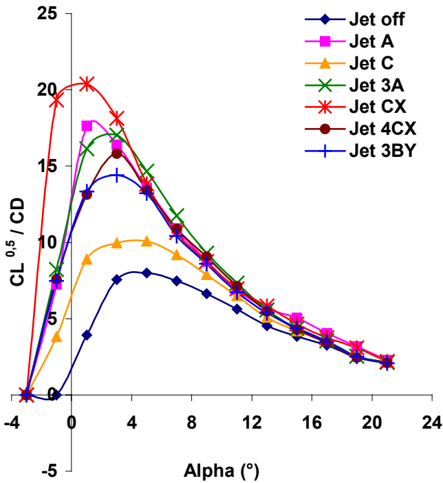
Figure 16 maximum range factor results of the best configurations.
