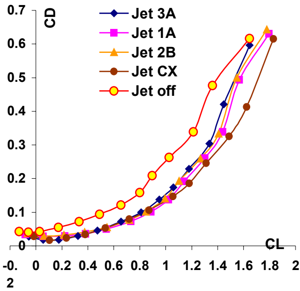
Figure 11 Drag polar for Double jets.
