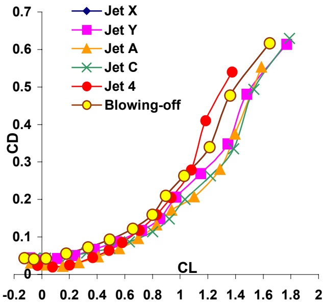
Figure 8 Single jet Drag polar.
