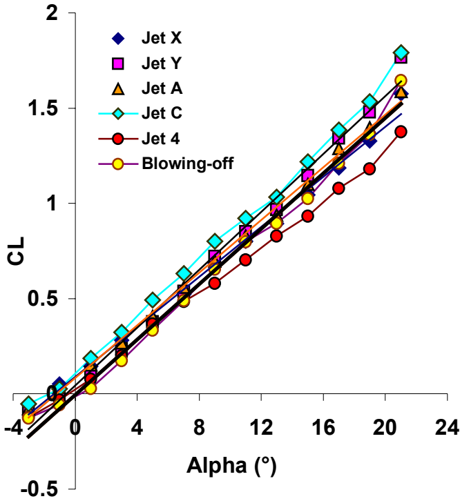
Figure 7 Single jet lift to alpha curves.
