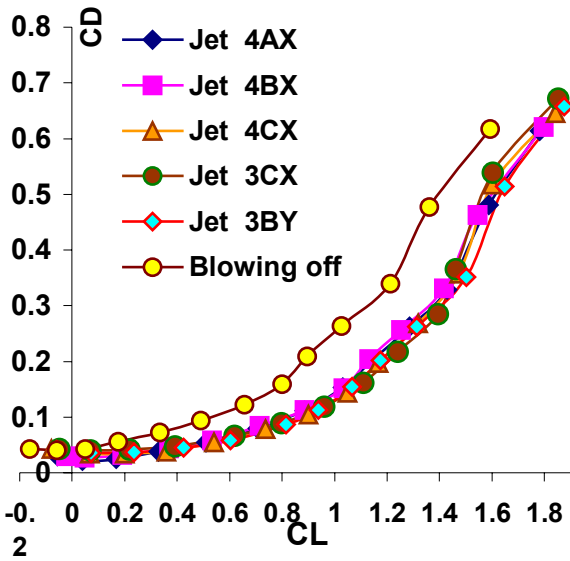
Figure 15 Drag polar for Triple Jets.
