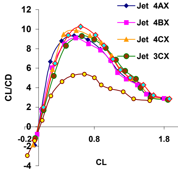
Figure 14 Wing efficiency with Triple Jets.
