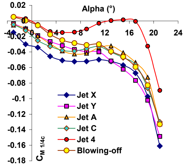
Figure 9 Pitching Moment results, Single Jets.
