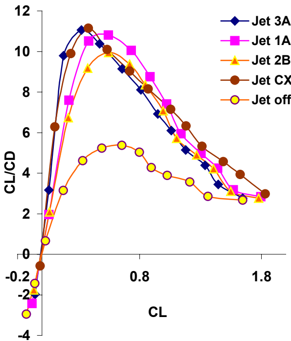
Figure 12 Wing efficiency with Double jets.
