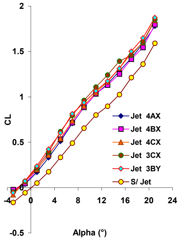
Figure 13 Lift curves for Triple Jets.
