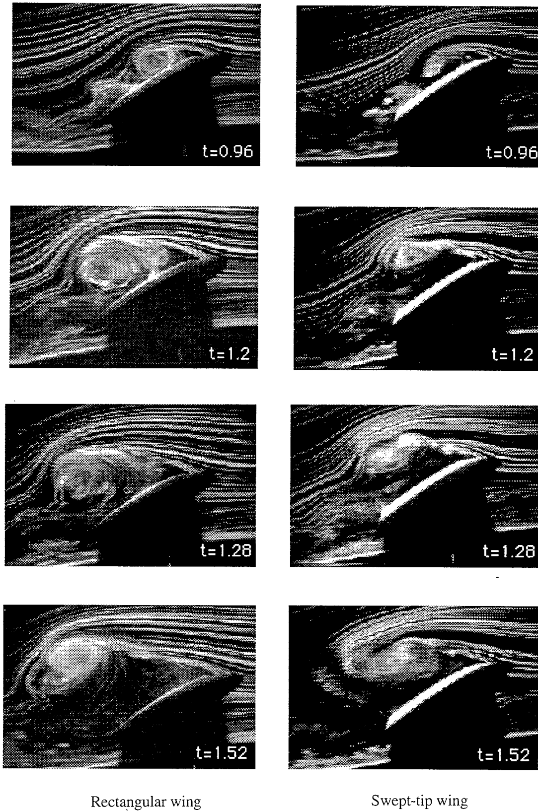
Fig. 7. Comparison of images from rectangular wing and rectangular wing with swept tips at 57% of span
