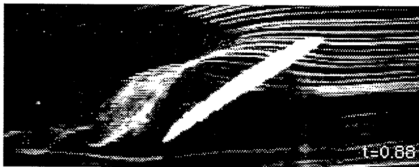
Fig. 9. Image recorded at 90% of span of rectangular wing with swept tips
