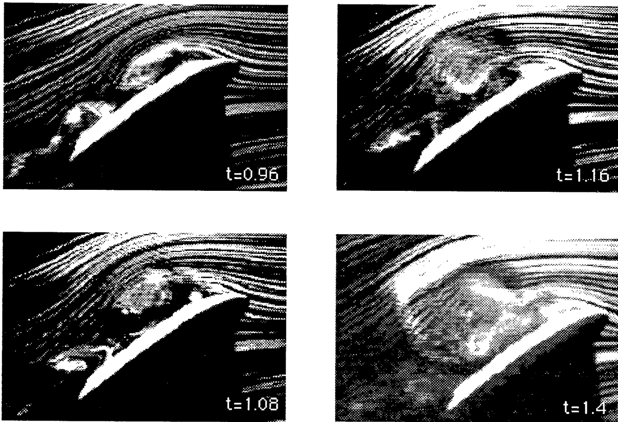
Fig. 8. Images recorded at 57% of span of rectangular wing with swept tips
