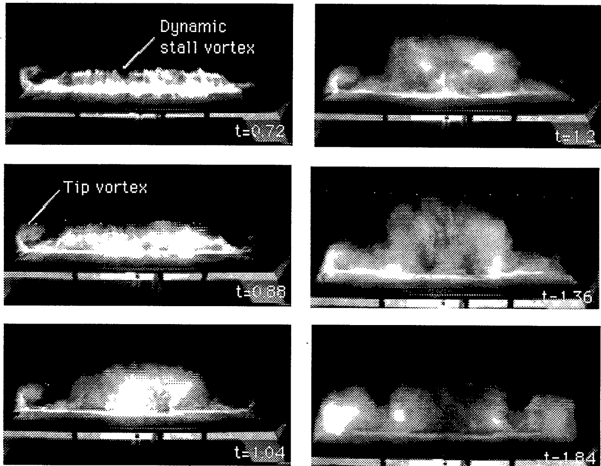
Fig. 6. View of rectangular wing from upstream
