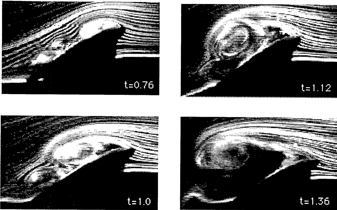
Fig. 3. Images recorded at 57% of span of rectangular wing
