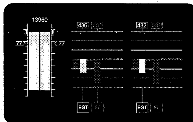
Figure 13 -- Erroneous Engine Pressure Ratio (EPR) Information, Task-Oriented Engine Display
