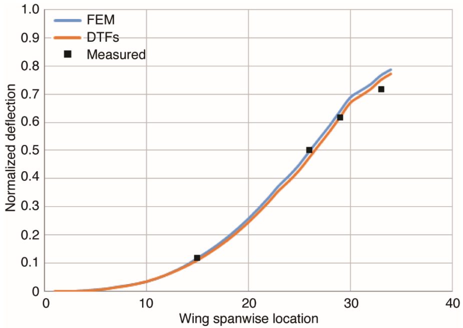
Fig. 10. Comparison of deflections along front strain-sensing lines.
