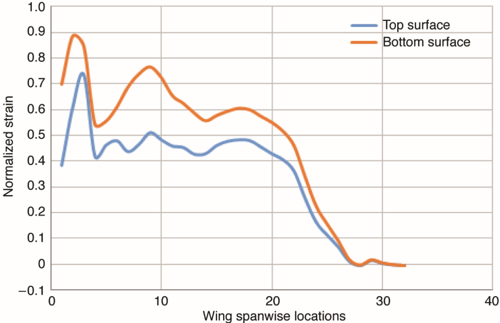
Fig. 7. Strain from the rear strain lines.
