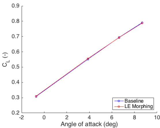
Fig. 8: Balance measurements with and without leading edge morphing
