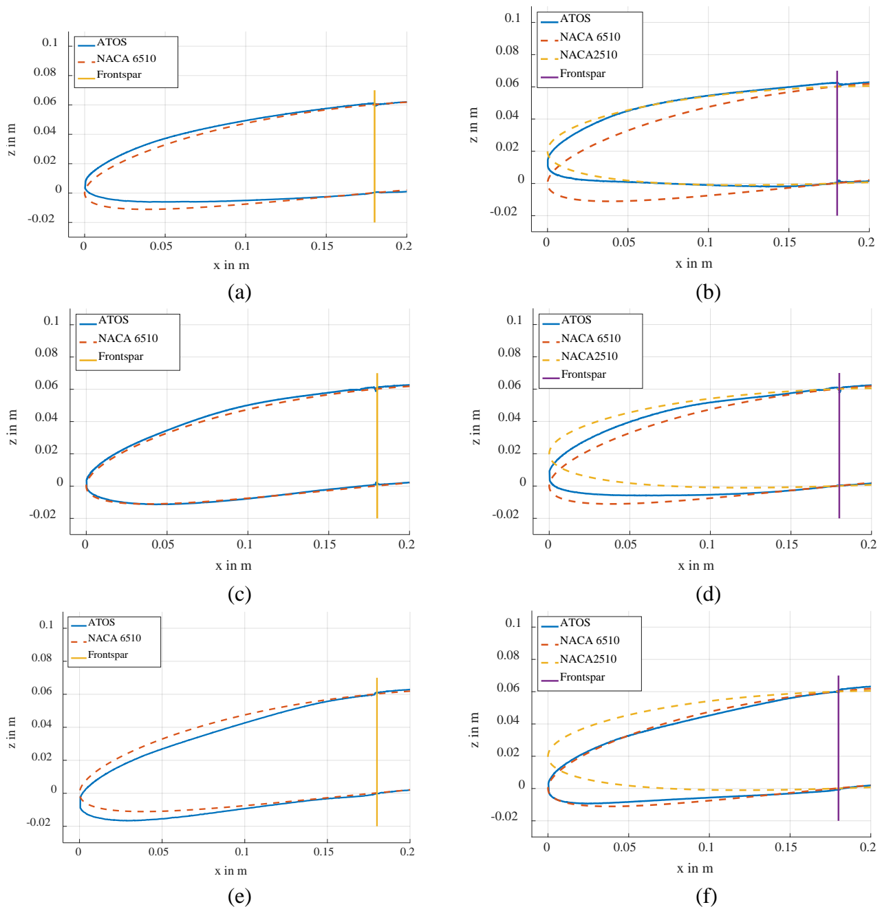
Fig. 13: Surface measurement for (a) baseline section S2, (b) morphed section S2, (c) baseline section S3, (d) morphed section S3, (e) baseline section S4, (f) morphed section S4
